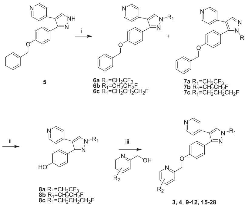
Scheme 1. Synthesis of final compounds 3, 4, 9–12, and 15–28 a
