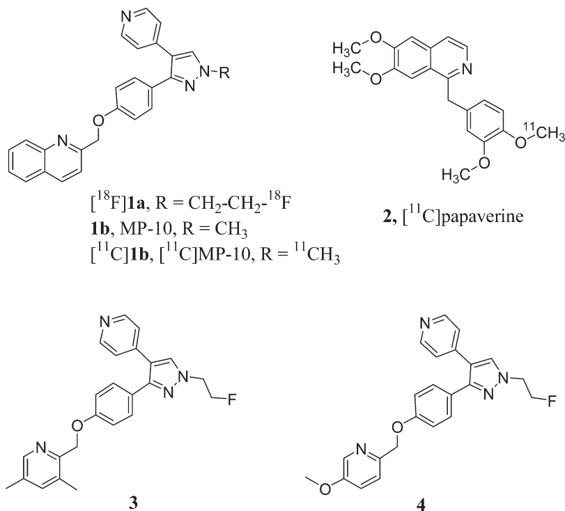
Chart 1. Structures of Some PDE10A Inhibitors and Derived PET Radioligands
