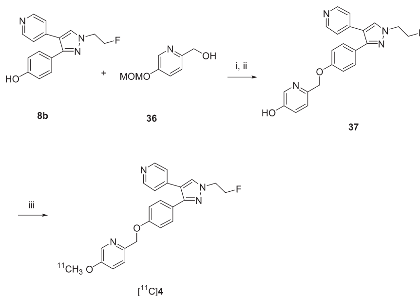
Scheme 5. Synthesis of Precursor 37 and Subsequent Radiosynthesis of [ ^{11}\text{C} ]4 a
