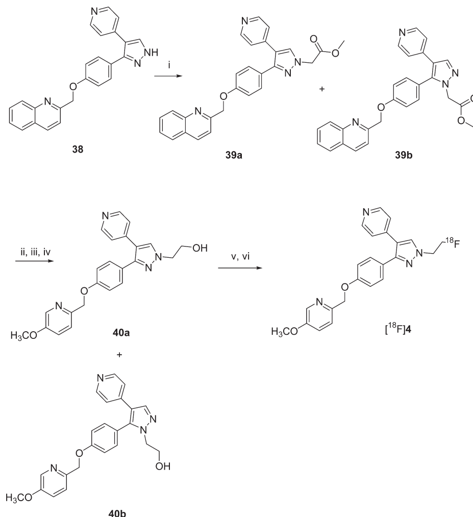
Scheme 6. Synthesis of Precursor 40a and Subsequent Radiosynthesis of [ ^{18}\text{F} ]4 a
