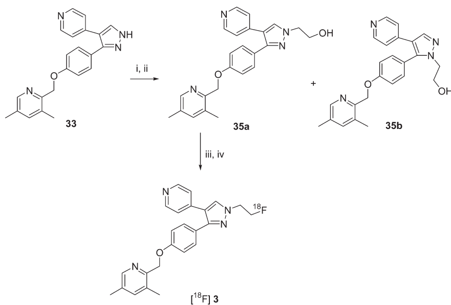
Scheme 4. Synthesis of Precursor 35a and Subsequent Radiosynthesis of [ ^{18}\text{F} ]3 a
