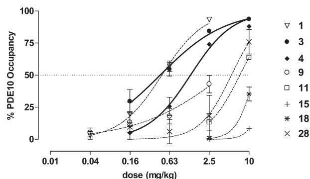
Figure 1. Dose-dependent occupancy of PDE10A in rat brain by different PDE10A inhibitors after sc administration using the radioligand [ 3 H]MP-10. Experimental details of the in vivo occupancy protocol are described in the Experimental Section. Bold curves highlight the two compounds ( 3 and 4 ) that were selected for radiolabeling and further investigation as potential PET ligands.
