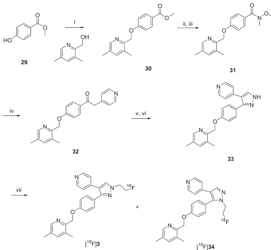
Scheme 3. Synthesis of Precursor 33 and Subsequent Radiosynthesis of [ ^{18}\text{F} ]3 a
